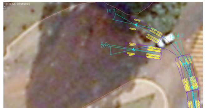
The vehicle swept path on the Mercedes Benz 6x4 illustrates the optimal path versus the path on a roundabout where the truck turned over.
